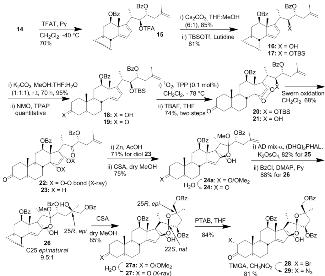
Scheme 2. Preparation of Cstat North 1 Azide, 29
